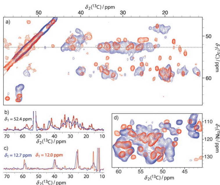
Figure 1. PDSD spectra of HET-s(218–289) fibrils formed at pH 3 (blue) and at pH 7 (red). (The complete spectra are shown in the Supporting Information.) a) Section of the aliphatic region. b, c) Slices through the C^\alpha region and at an isoleucine C^\beta resonance to clarify the differences in observed linewidths. d) Section of the ^{15}\text{N} – ^{13}\text{C} HETCOR spectrum. All spectra were recorded with a mixing period of 50 ms and 90 kHz SPINAL-64 ^1\text{H} decoupling during t_1 and t_2 at a static magnetic field of 14.09 T.
