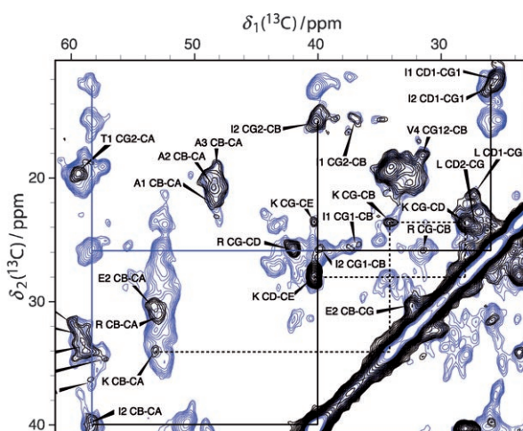
Figure 2. Sections of the ^{13}\text{C} – ^{13}\text{C} TOBSY (black) and 50 ms PDSD (blue) spectra of the pH 3 fibrils. The solid black and blue lines connect cross peaks belonging to I_2 in the TOBSY and the PDSD spectrum, respectively; the dotted black line follows cross peaks of the K spin system. The assignments were obtained by analysis of the TOBSY, PDSD, and N–C HETCOR spectra; the spin systems were numbered arbitrarily. The spectra shown were recorded at 13 kHz MAS with 90 kHz SPINAL-64 ^1\text{H} decoupling during t_1 and t_2 . The mixing times were 5 ms and 50 ms for the TOBSY and the PDSD spectra, respectively.
